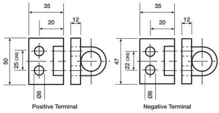
TM Marine Dual Terminals
