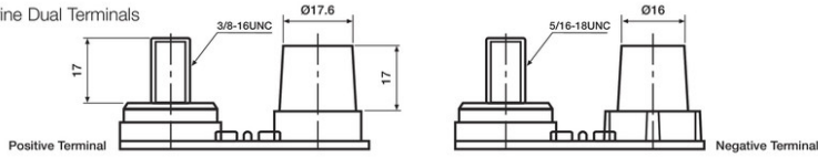
TM Marine Dual Terminals
