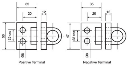
TM Marine Dual Terminals
