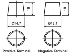
T3 Small Japanese JIS Terminal
